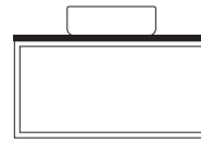
80cm Wall Hung Single Unit 800(w) x 402(h) x 455(d)mm (Excl. Basin) One soft close drawer
