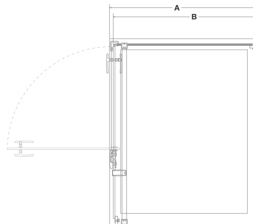
Frameless side panel
