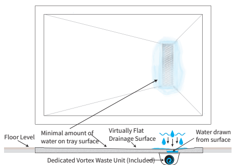
Linear Waste Shower Tray
