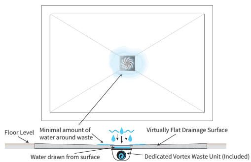
Central Waste Shower Tray
