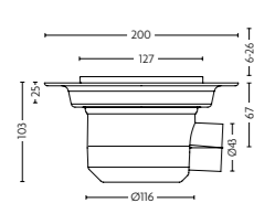
Tiled Floor Gully - Horizontal Outlet
